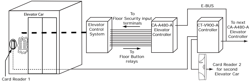
Figure 7: Security Enabling Control:
